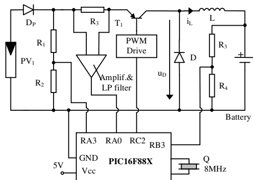
Fig.7. Conversion system
