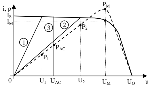
Fig.4. Level of power supplied by a PV for different loads
