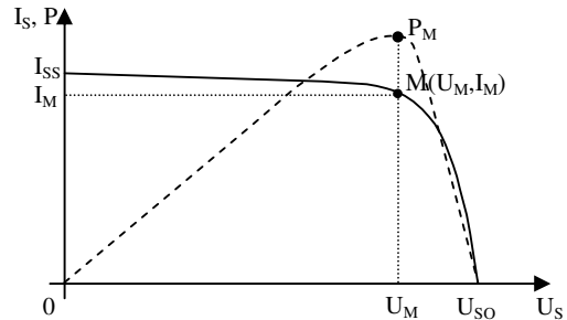
Fig.2. Maximum power point for a silicon solar cell
