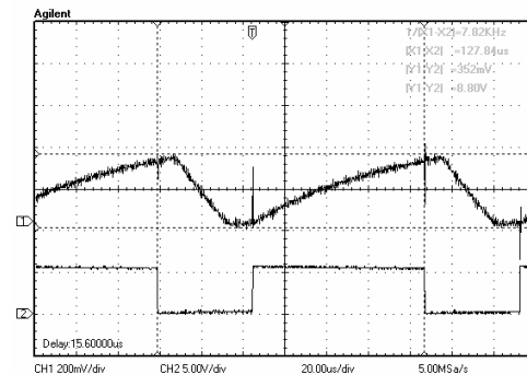
Fig.8. Below - command voltage and above - the u_D voltage at 0.3KW/m^2 irradiance
