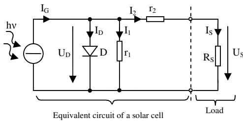
Fig.1. Model of a solar cell
