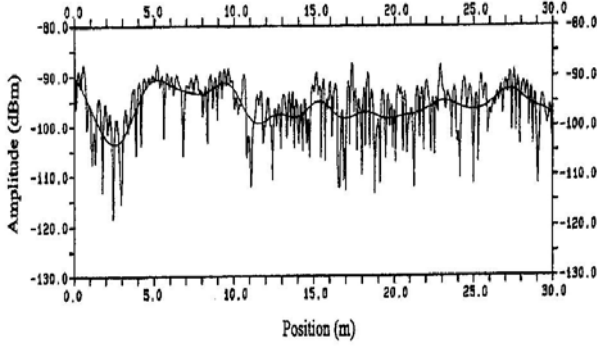
Fig. 2. Amplitude of the received signal as a function of the range dependence. Here the slow and fast fading are represented.
