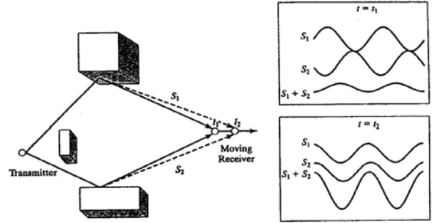
Fig. 3. Representation of constructive and destructive interference between two signals. The key role is played by the phase difference between S_1 and S_2 .
