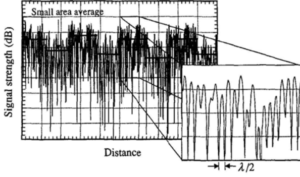
Fig. 4. Small-area obtained by averaging over discrete intervals. How the fast fading can be separate out from the slow fading.
