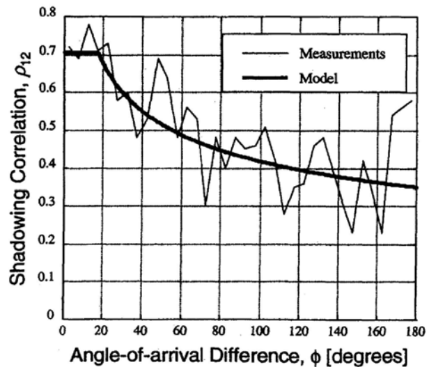
Fig.10. Comparison of measurements and model for shadowing cross-correlation.
