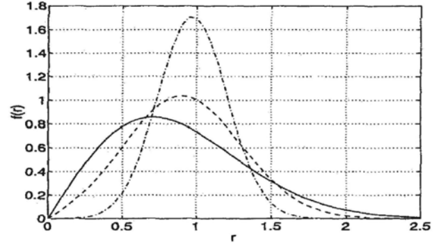
Fig. 5. Ricean probability density function, (-) K=\infty , (--) K=3(\text{db}) (-.-) K=9(\text{db})
