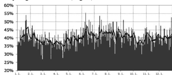
Fig. 3 Average differences of daily mean wind velocities from the 50-year daily average in Western Hungary grid
